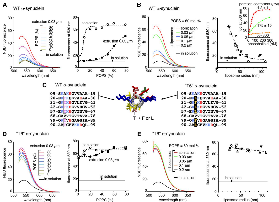
Figure 3. The ability of \alpha -synuclein to sense the curvature of negatively charged lipid membranes depends on its poorly developed hydrophobic face.
